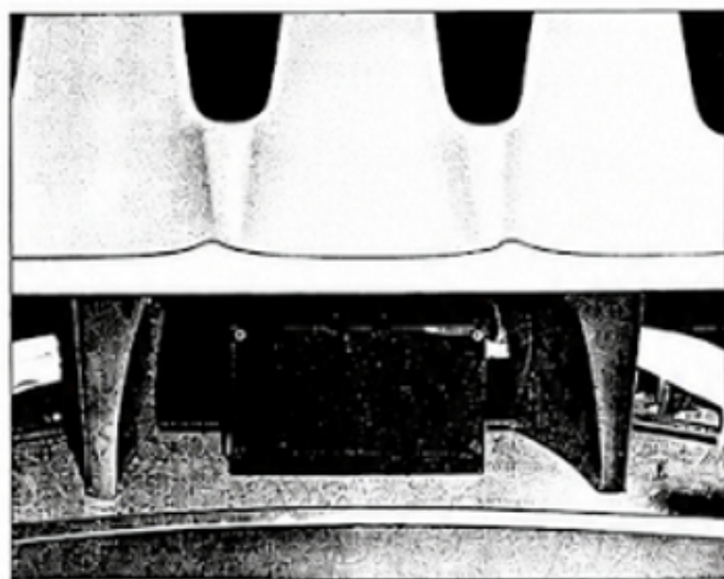
Fig. 9.—Sound reproducing units (left) are located under every third seat. Power for these units is picked up through a double brush collector (right) at every sixths seat. The collector rides in an electrical feed rail attached to the side of the track. The rail runs the entire length of the track.
